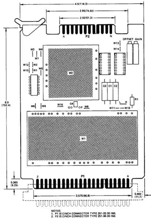
Figure 12. AC1580 Mounting Board
