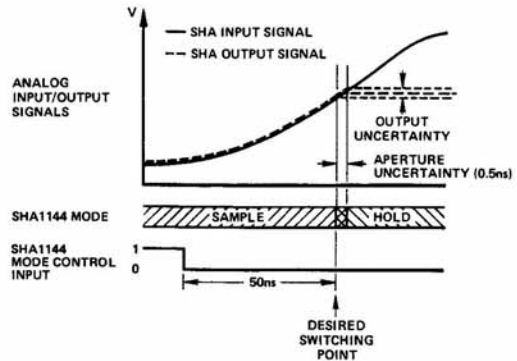
Figure 4. Aperture Uncertainty
