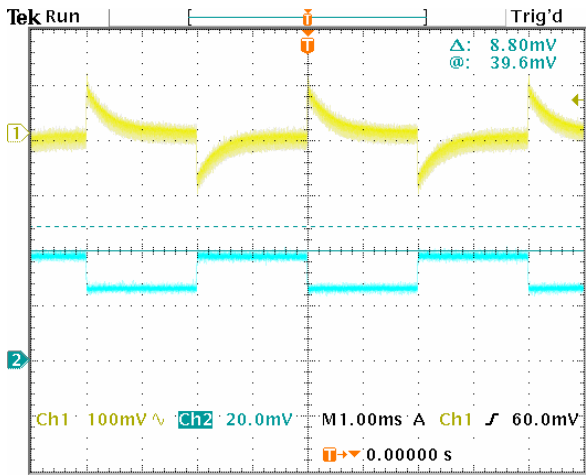
Fig 13. Dynamic response of load step at V_{in}=48v , Ch1: output voltage (100mv/div), Ch2: output current step of 50%-75%-50% (2A/div). Current slew rate: 0.1A/\mu s , C_o=10\mu F tantalum capacitor + 1\mu F Ceramic capacitor, time scale: 1ms/div
