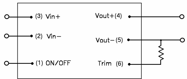
Fig 2. Configuration for increasing the output voltage
