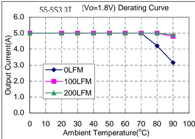
Figure 10c. Typical Power De-rating for 5.0V IN 1.8Vout
