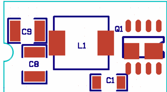
Figure 9. Temperature Measurement Location for SMT
