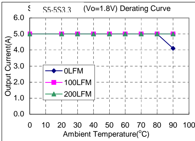
Figure 13c. Typical Power De-rating for 3.3V IN 1.8Vout
