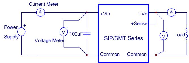
Figure 15. S5 Series Test Setup
