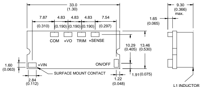
Figure 16. S15-5S3.3 Mechanical Outline Diagram
