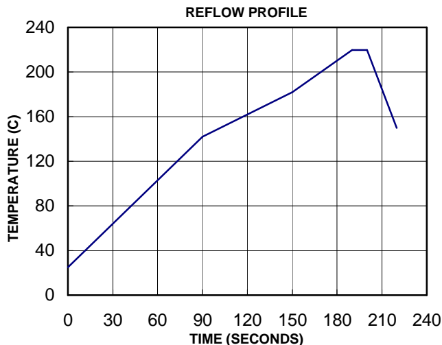
Figure 14 – SMT Reflow Profile
