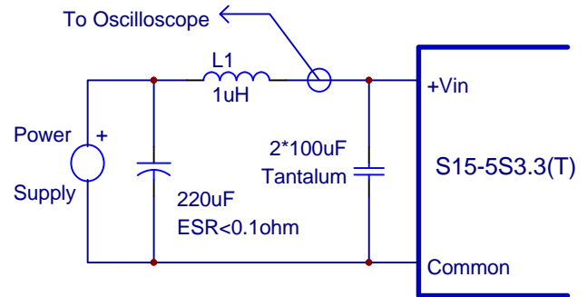
Figure 9. Input Reflected-Ripple Test Setup
