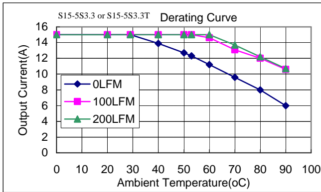
Figure 7. Typical Power De-rating for 5.0V IN(SIP15)
