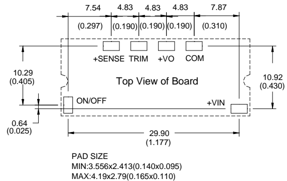
Figure 4B. Recommended SMT Footprint
