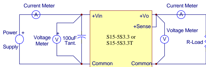
Figure 10. S15-5S3.3 Test Setup
