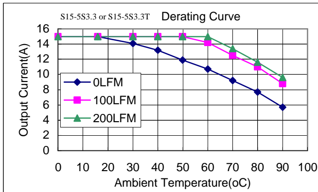
Figure 8. Typical Power De-rating for 5.0V IN (S15-5S3.3)
