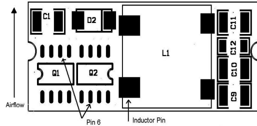
Figure 6B. Temperature Measurement Location for SMT
