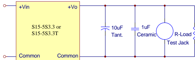
Figure 13. Output Voltage Ripple and Noise Measurement Set-Up
