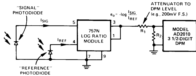
Figure 6. Model 757N Applied to Absorbance Measurements
