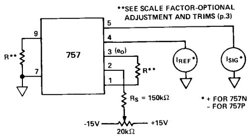
Figure 3. Output Voltage Offset Adjustments
